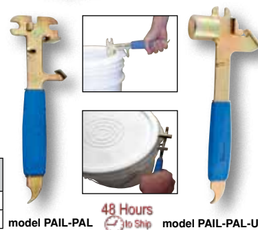
model PAIL-PAL model PAIL-PAL-UN
