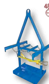
model CYL-P-6-LUG
