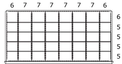
40 Compartments
