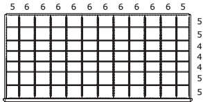
0504 84 compartments
