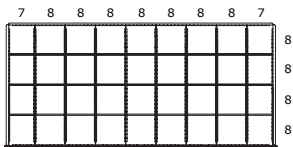
0808 36 compartments
