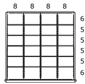
0805 24 compartments
