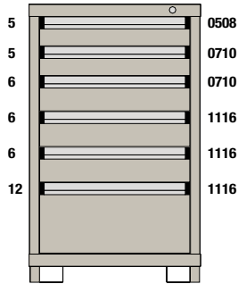
M1-232940FT-MD06CL 6 Drawers 46 Compartments
