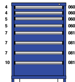
M1-302949FT-MD08CL 8 Drawers 148 Compartments
