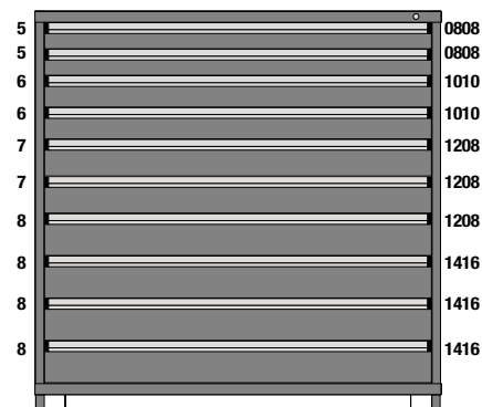
M1-602968FT-MD10BL 10 Drawers 216 Compartments
