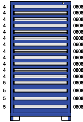
M1-302968FT-MD16AL 16 Drawers 296 Compartments
