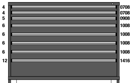
M1-602949FT-MD08AL 8 Drawers 234 Compartments
