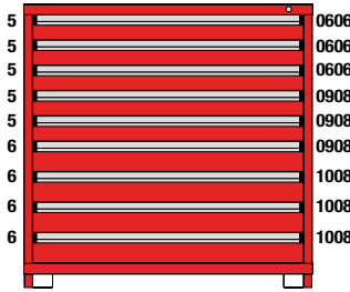
M1-452949FT-MD09CL 9 Drawers 267 Compartments
