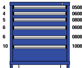
M1-302935FT-MD06CL 6 Drawers 108 Compartments
