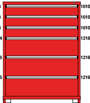
M1-452968FT-MD06AL 6 Drawers 69 Compartments
