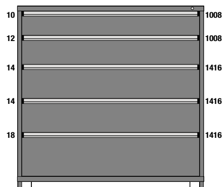
M1-602968FT-MD05AL 5 Drawers 86 Compartments
