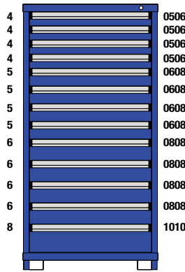
M1-302968FT-MD13BL 13 Drawers 273 Compartments
