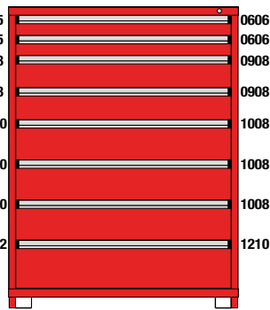
M1-452968FT-MD08AL 8 Drawers 190 Compartments
