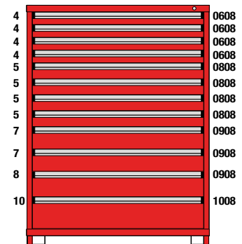
M1-452968FT-MD12AL 12 Drawers 348 Compartments
