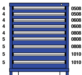
M1-302940FT-MD09DL 9 Drawers 154 Compartments
