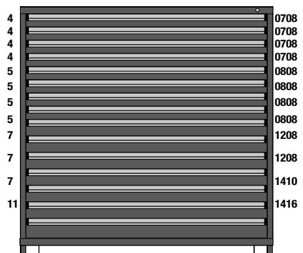
M1-602968FT-MD15AL 15 Drawers 543 Compartments
