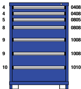
M1-302949FT-MD07AL 7 Drawers 137 Compartments
