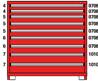
M1-452949FT-MD09AL 9 Drawers 254 Compartments
