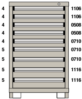
M1-232940FT-MD09AL 9 Drawers 91 Compartments
