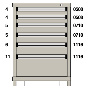
M1-232935FT-MD06CL 6 Drawers 58 Compartments
