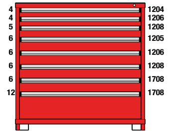
M1-452949FT-MD08AL 8 Drawers 152 Compartments
