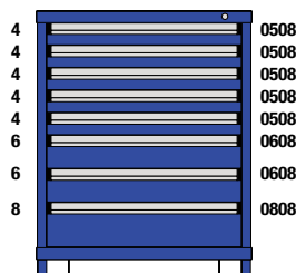
M1-302940FT-MD08DL 8 Drawers 176 Compartments
