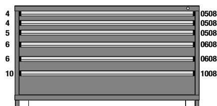
M1-602935FT-MD06AL 6 Drawers 284 Compartments
