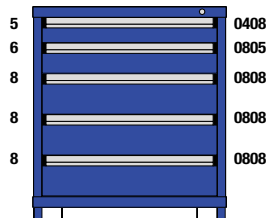
M1-302935FT-MD05AL 5 Drawers 104 Compartments
