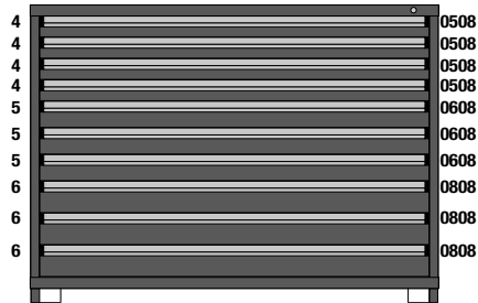
M1-602949FT-MD10AL 10 Drawers 464 Compartments
