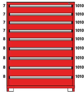
M1-452968FT-MD09CL 9 Drawers 135 Compartments
