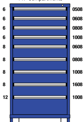
M1-302968FT-MD09EL 9 Drawers 140 Compartments
