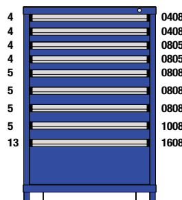
M1-302949FT-MD09CL 9 Drawers 180 Compartments
