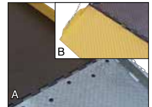
A) ALUMINUM BRIDGE • WL-SATB B) STEEL BRIDGE (add'l) • WL-SSTB
