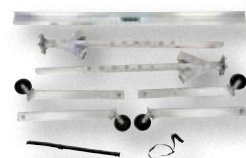
KNOCKDOWN DESIGN FOR EASY TRANSPORTATION ONTO ROOFS OR THROUGH DOORWAYS
